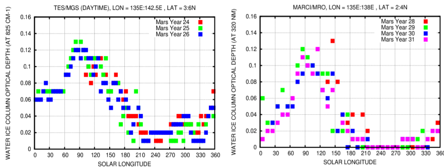
Fig. 5 Seasonal evolution of the water ice clouds observed during daytime above the InSight landing site. Top : Cloud opacity at 12.1 \mu\text{m} ( 825 \text{ cm}^{-1} ) at about 2pm local time as retrieved by Smith (2004) from the MGS/TES observations. Bottom : Cloud daytime UV opacity at 0.320 \mu\text{m} as retrieved by Wolff et al. (2014) from the MRO/MARCI observations. Assuming simple spherical shapes for water ice particles with effective radius 3 microns, the TES opacity at 12.1 \mu\text{m} can be converted to the MARCI opacity at 0.320 \mu\text{m} by multiplying by a factor \sim 1.86 [ 1.37 to account for the absorption (TES) vs. extinction (MARCI) difference (Wolff and Clancy 2003) and 1.36 to account for the wavelength difference (Clancy et al. 2003)]. Note that water ice opacity has also been retrieved from several other instruments (e.g. THEMIS, PFS): only TES and MARCI results are shown here for the sake of simplicity.
